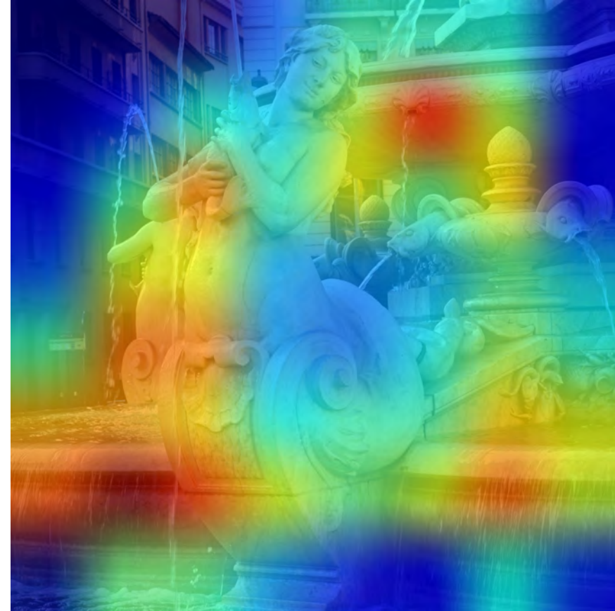
Grad-CAM
