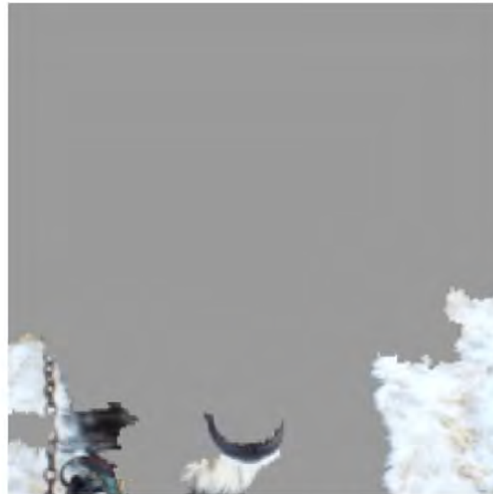
(b) Explanation
