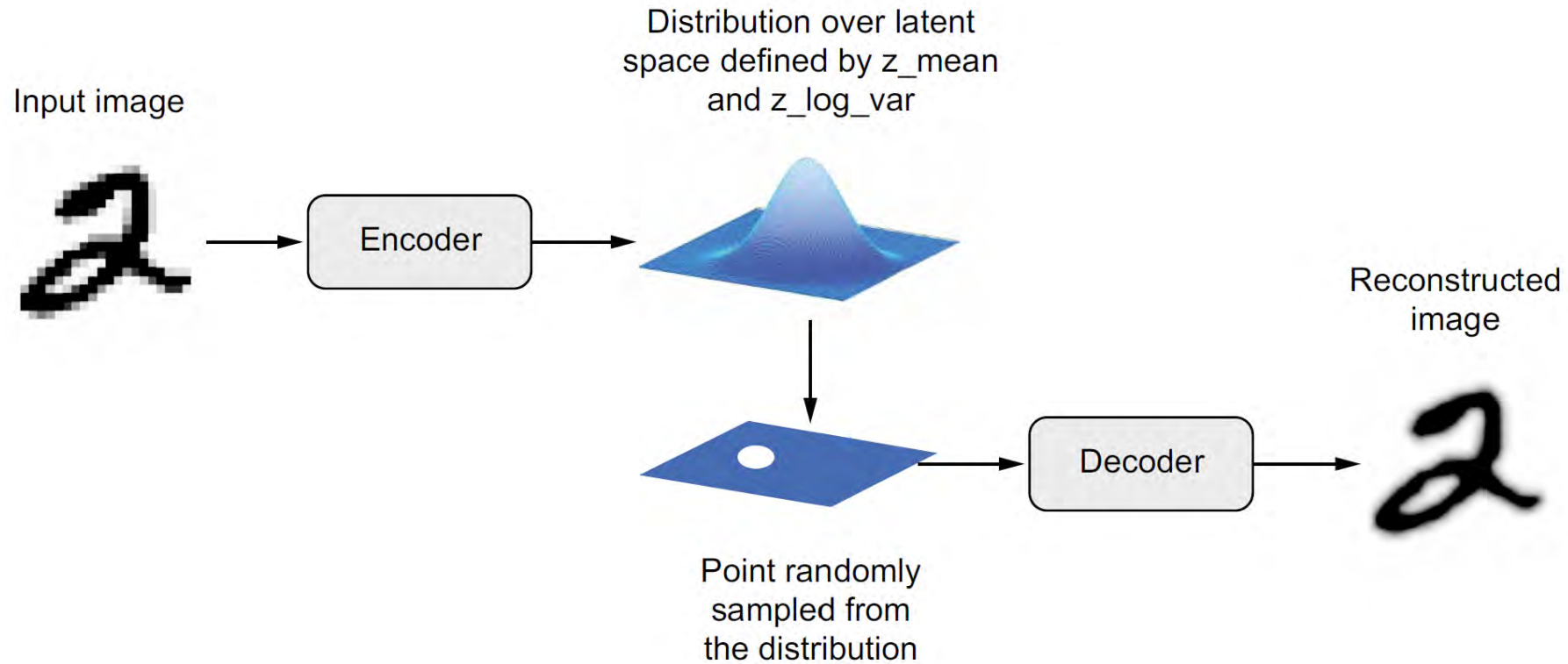
Schematic of a variational autoencoder.
